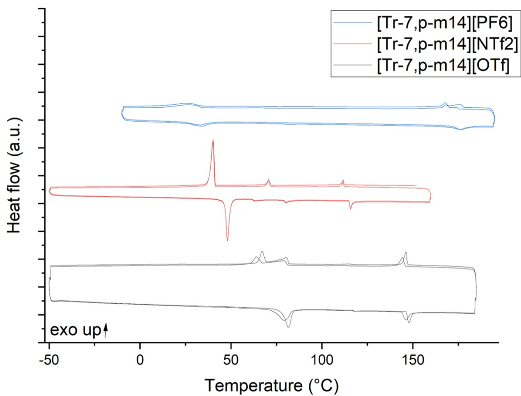
Figure S1 | DSC analysis of the p-m substituted OTf, PF 6 - and NTf 2 - triazolium salts, highlighting the multistep mesophase behavior, the counterion-dependent transition profiles, and the reproducibility across multiple heating-cooling cycles.
